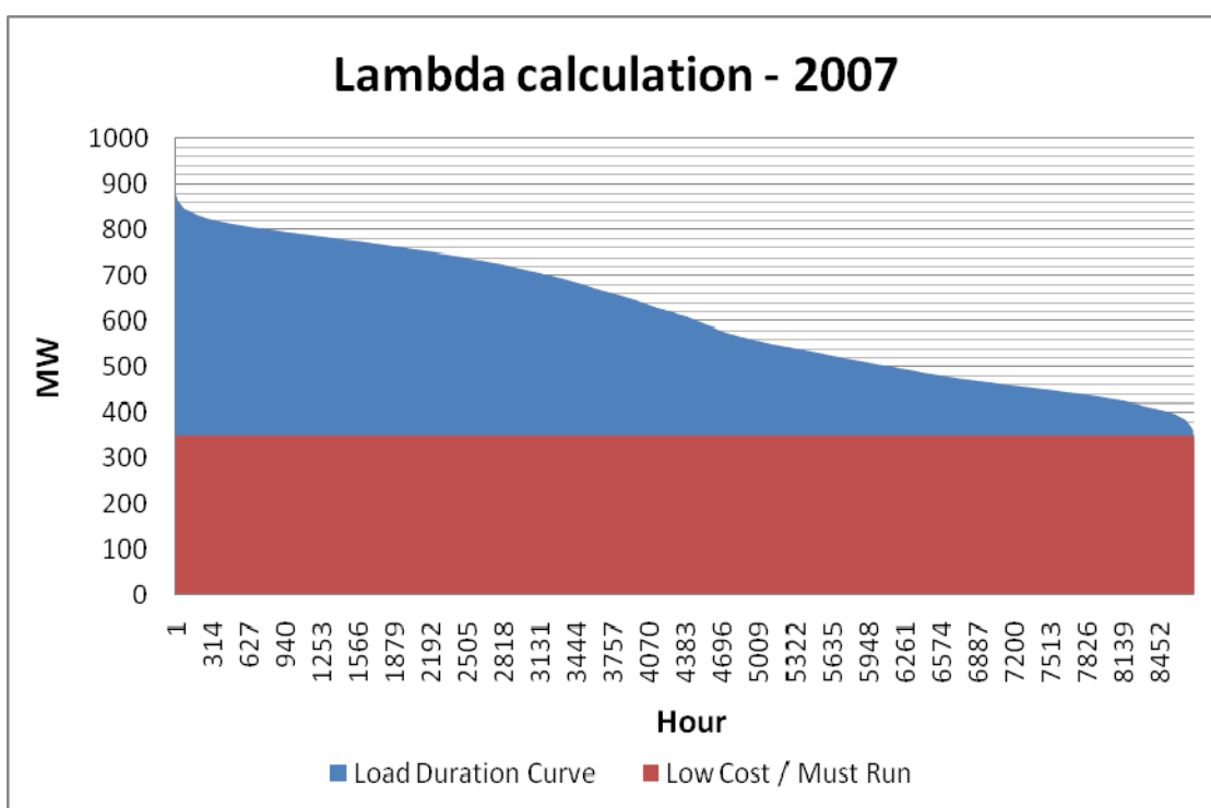
Salvadorean Load Duration Curve – 2007
