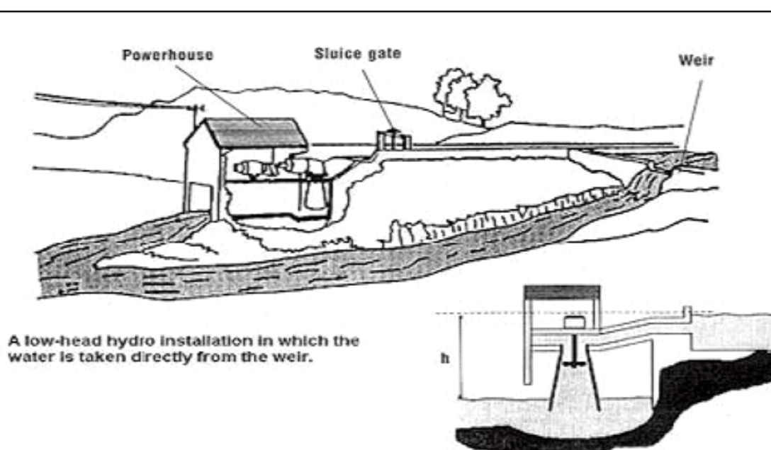
Figure 1. Schematic view of a run-of-river power plant
