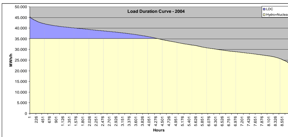
Figure 12 – Load duration curve for the S-SE-CO system, 2005
